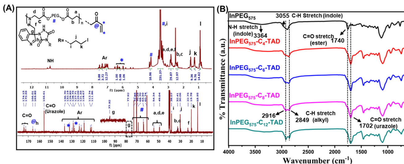
Fig. 3 (A) ^1\text{H} - and ^{13}\text{C} -NMR spectra of \text{InPEG}_{575}\text{-C}_4\text{-TAD} and (B) FTIR spectra of \text{InPEG}_{575} and \text{InPEG}_{575}\text{-C}_n\text{-TAD} ( n = 4, 6, 8, 12 ).
