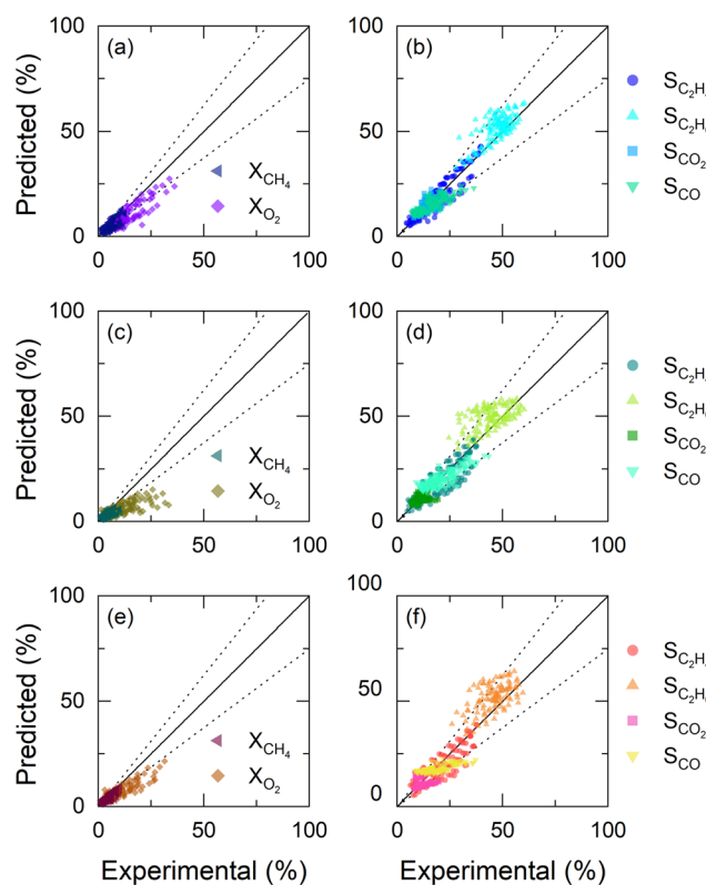
Fig. 6 Parity plots obtained by fitting experimental performance metrics to the microkinetic model with the descriptors in Table 5 for (a and b) IMP SiO 2 , (c and d) SD SiO 2 -α + βSiC, and (e and f) SD SiO 2 -βSiC.
