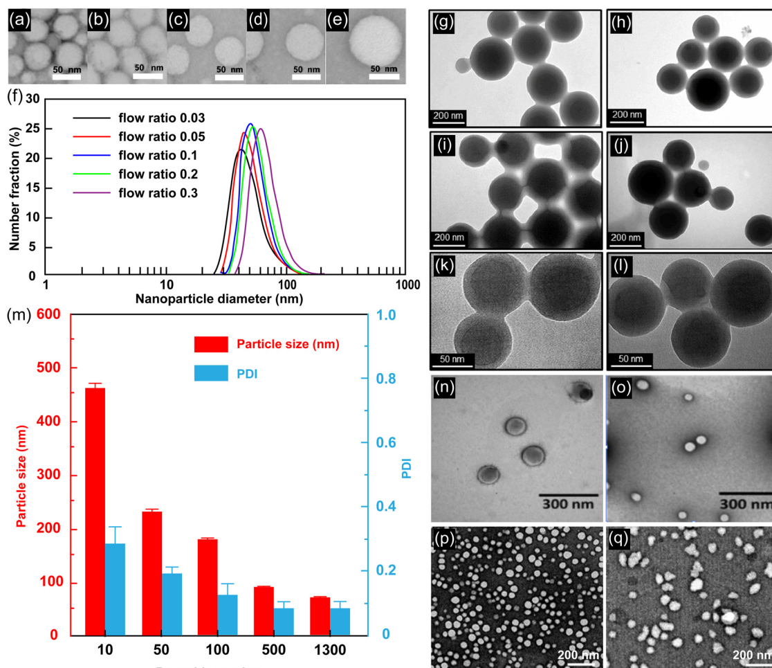
Fig. 5 (a)–(e) TEM images of PNP prepared at flow rate ratios. The PNP of mPEG-PLGA from the flow ratios of (a) 0.03, (b) 0.05, (c) 0.1, (d) 0.2, (e) 0.3. (f) Corresponding dynamic light scattering plots of PNP. 81 (g)–(l) TEM images of the core-shell PNP synthesized by varying drug-polymer weight ratio and Reynolds number. (g) and (h) Drug-polymer weight ratio of 1:1 and Re of 100. (i) and (j) Drug-polymer weight ratio of 2:1 and Re of 100. (k) and (l) Drug-polymer weight ratio of 1:1 and Re 1300. (m) Particle size distribution and polydispersity index (PDI) as a function of Reynolds number. 82 (n) and (o) TEM images of PNP prepared under varying flow rate ratios of (n) 1:1 and (o) 10:1. 59 (p) and (q) TEM images of PNP as a function of drug (curcumin) to polymer ratio at (p) 0.5 and (q) 10. 5
