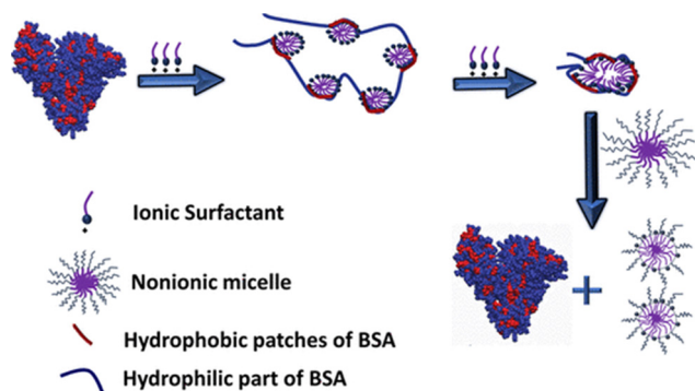
Fig. 4 Schematic showing the unfolding of BSA protein in the presence of ionic ( C_n TAB; n = 10, 12, 14 and 16 ) surfactants and then refolding upon further addition of nonionic (C12E10) surfactants at pH 7. All tested cationic surfactants induce BSA unfolding, where the denatured state is depicted as a beads-on-a-string configuration, consistent with a random flight model. Upon subsequent addition of the nonionic surfactant, C12E10, mixed micelles are formed, which effectively sequester the ionic surfactant away from the protein. Reproduced from ref. 12 with permission from the American Chemical Society, copyright 2018.
