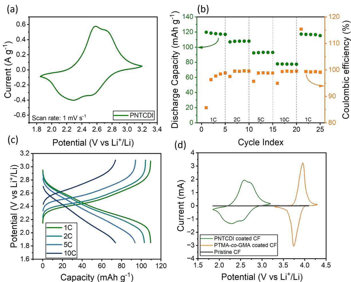
Figure 2. Electrochemical characteristics of PNTCDI-coated CF in a half cell (vs lithium foil) at room temperature ( 24^\circ\text{C} ). (a) CV at 1 \text{ mV s}^{-1} . (b) Discharge capacity at varying C-rates. (c) GCD curves at different C-rates. (d) CV curves of PNTCDI, PTMA-co-GMA, and neat CF shown together. The electrolyte was 1 M LiTFSI in diglyme/FEC (9:1, w:w). All cells had an active material loading of >1 \text{ mg cm}^{-2} .
