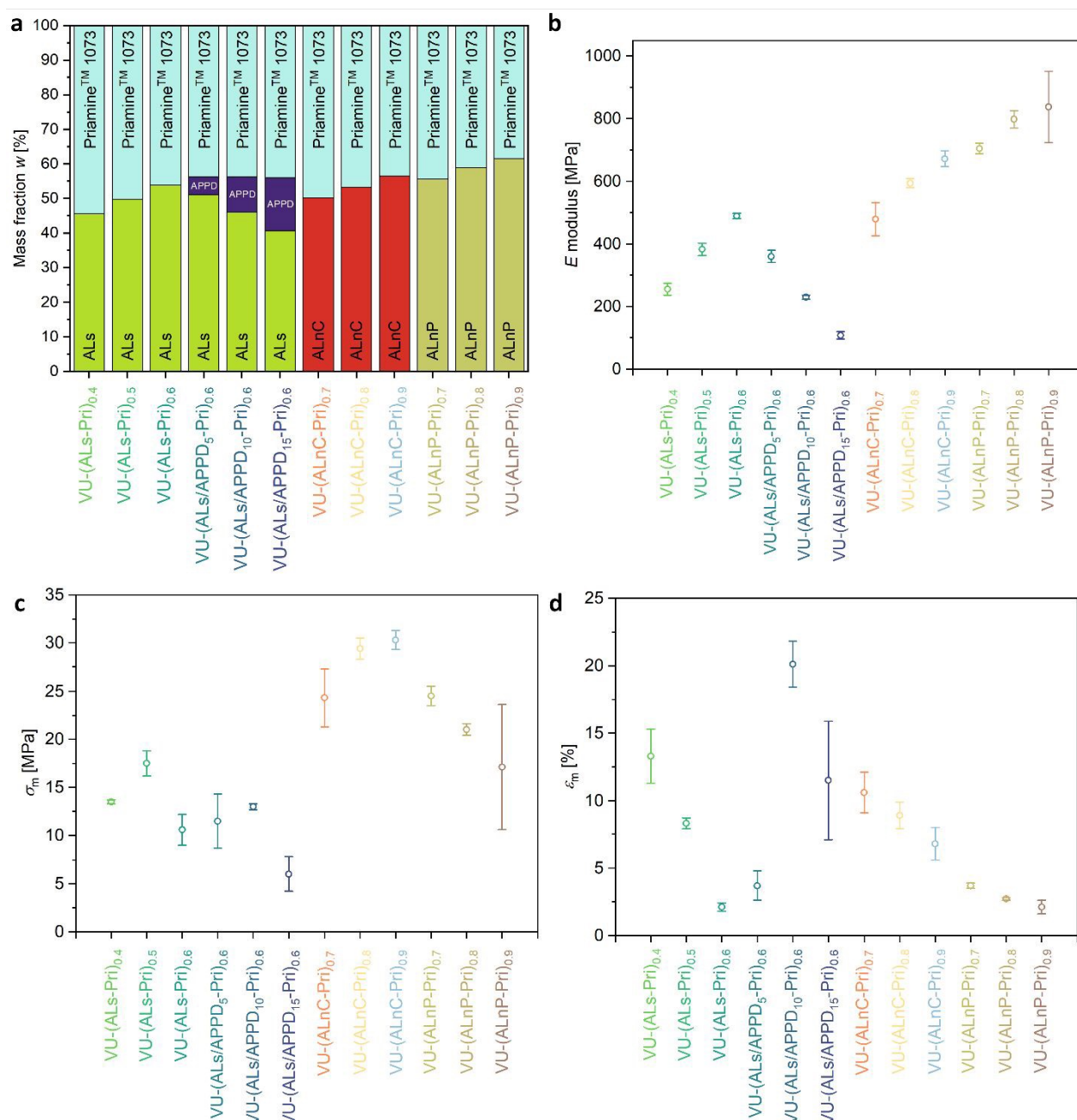
Figure 3: (a) Mass fractions of the used building blocks of the lignin vitrimers with the acetoacetylated lignin species ALs, ALnC, and ALnP, respectively, the linear difunctional APPD, and the amount of Priamine™ 1073. (b-d) Tensile test data of the lignin vitrimers ( T = 23 °C), (b) Tensile modulus ( E ), (c) Tensile strengths ( \sigma_m ), (d) Elongation at ultimate stress ( \epsilon_m ).
