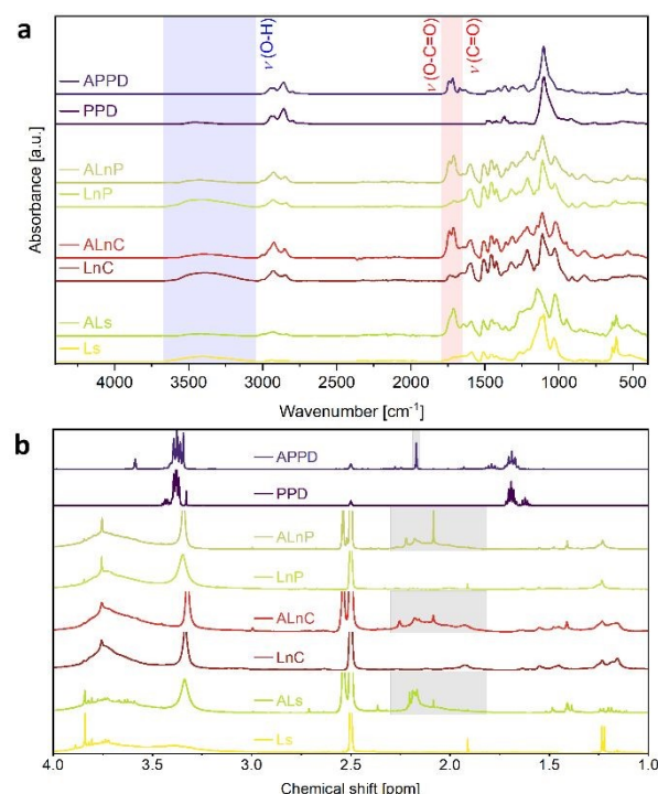
Figure 1: (a) ATR-FT-IR spectra of the different lignin sources (Ls, LnC, and LnP), as well as of Poly(oxy-1,3-propanediyl) (PPD) and the respective acetoacetylated species (ALs, ALnC, ALnP, and APPD) showing the characteristic bands of the acetoacetate group with the C=O ester (1735 – 1741 cm -1 ) and C=O ketone (1712 – 1716 cm -1 ) stretching vibration bands. The lignin backbone represents the C–O (995 – 1148 cm -1 ), C–C (2850 – 3050 cm -1 ), C=C (1148 – 1650 cm -1 ), and O–H (3050 – 3650 cm -1 ) stretching vibration bands. (b) 1 H NMR spectra of PPD, LnP, LnC, and Ls, as well as the acetoacetylated APPD, ALnP, ALnC, and ALs, showing the characteristic chemical shift of the acetoacetate groups (grey) (400 MHz, 298 K, DMSO- d 6 ).
