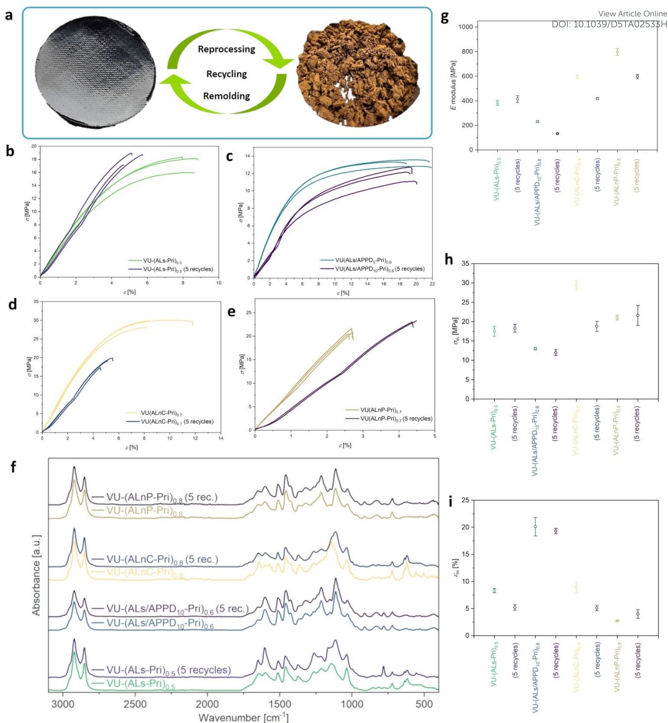
Figure 6: (a) Illustration of the repetitive ball milling (1 min, f = 30 Hz, T = 23 °C) and reprocessing cycle through heat compression (30 min, 20 kN, 180 °C), showing a ground lignin vitrimer powder and a reprocessed vitrimer film. Stress-strain curves ( T = 23 °C) of selected vitrimers VU-(ALs-Pri) 0.5 (b), VU-(ALs/APPD 10 -Pri) 0.6 (c), VU-(ALnC-Pri) 0.8 (d) and VU-(ALnP-Pri) 0.8 (e) in comparison of the pristine and five times reprocessed specimens, showing different curves with overall similar material properties. (f) Repetitively measured ATR-FT-IR spectra show rather similar curve shapes of the pristine materials and after five times recycling procedure, measuring the characteristic stretching vibrations of the vinylous urethane bond. (g-i) Tensile test data of the pristine and five times reprocessed lignin vitrimers ( T = 23 °C), (g) E modulus, (h) Tensile strengths ( \sigma_m ), (i) Elongations at ultimate stress ( \epsilon_m ).
