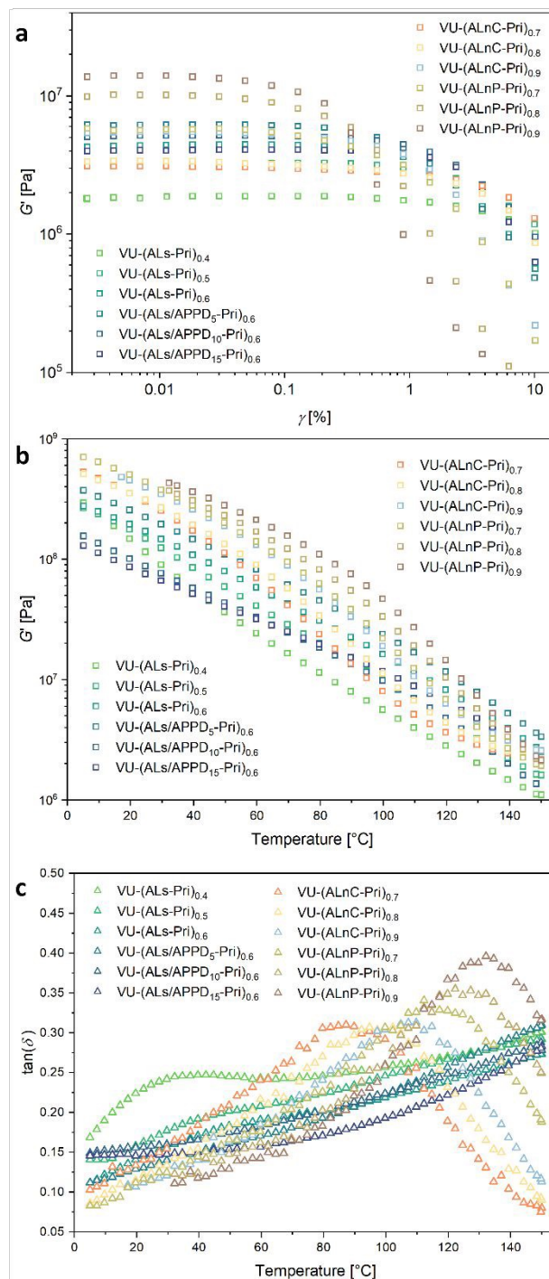
Figure 4: DMA results of the lignin vitrimers based on lignosulfonate and enzymatic lignins ( \omega = 6.28 \text{ rad s}^{-1} , F_N = 1 \text{ N} ). (a) Amplitude-sweep measurement results of the tested lignin vitrimers ( T = 110 °C). (b, c) Temperature-sweep measurements of the lignin vitrimers. ( T = 150 - 0 °C, \gamma = 0.01\% ), (b) Storage modulus G' , (c) Loss factor \tan(\delta) .
