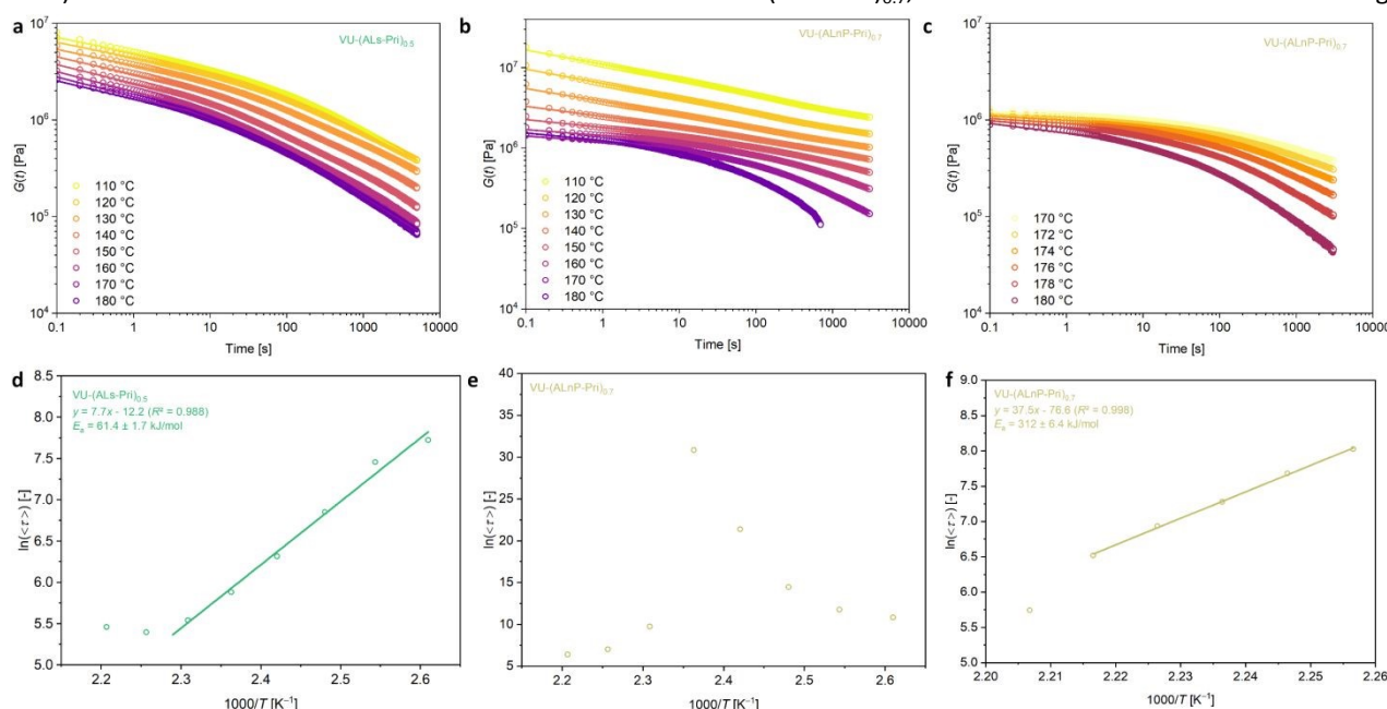
Figure 5: Non-normalized stress-relaxation measurement ( \gamma = 1\% , F_N = 1\text{ N} ) between 110 °C and 180 °C of the material (a) VU-(ALS-Pri) 0.5 and (b) VU-(ALnP-Pri) 0.7 . (c) Non-normalized stress-relaxation measurement ( \gamma = 1\% , F_N = 1\text{ N} ) between 170 °C and 180 °C of the material VU-(ALnP-Pri) 0.7 . (d-e) Arrhenius plot of \ln(\tau_r) versus 1000/T . For VU-(ALnP-Pri) 0.7 , a non-linear plot (e) was found due to the high T_g of the lignin particles in the range of 110 – 180 °C. A linear stress-relaxation relation could be found for VU-(ALnP-Pri) 0.7 in the range of 170 – 180 °C (f).
