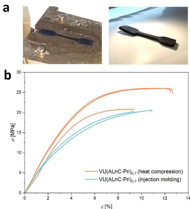
Figure 7: (a) Pictures of the injection mold and the produced test specimen. (b) Comparison of the stress-strain curves specimens produced through heat compression and through injection molding.
