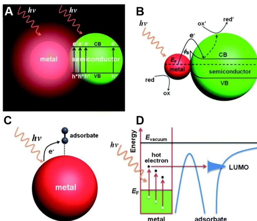
Fig. 3 Schematic representation of the three primary mechanisms by which plasmons facilitate light-driven chemical reactions. (A) Plasmon-enhanced light absorption through intensified near-field effects. (B) Plasmonic sensitization of the semiconductor via hot carrier injection. (C, D) Direct photocatalysis on pure metal surfaces driven by plasmon excitation. VB and CB represent the valence band and conduction band of the semiconductor, respectively. E_F denotes the Fermi level at equilibrium. “red” and “ox” indicate the reduced and oxidized forms of a chemical species, respectively. E_{vacuum} refers to the vacuum energy level. Reproduced with permission from ref. 64. Copyright 2013 Royal Society of Chemistry.
