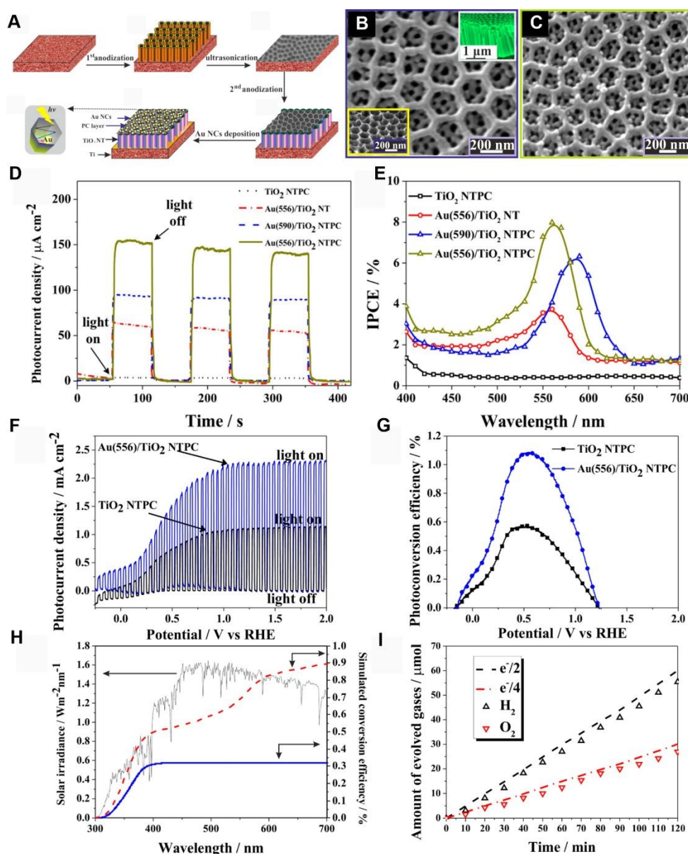
Fig. 10 (A) Schematic diagram of the Au/ \text{TiO}_2 nanotube photonic crystal fabrication procedure. SEM images of (B) \text{TiO}_2 nanotube photonic crystal and (C) Au/ \text{TiO}_2 nanotube photonic crystal. (D) Amperometric I-t curves at an applied potential of 1.23 V vs RHE under illumination of visible light with wavelength \geq 420 nm with 60 s light on/off cycles. (E) IPCE plots in the range of 400–700 nm at 1.23 V vs RHE. (F) Photoelectrochemical performance of various \text{TiO}_2 -based platforms. Linear sweep voltammograms recorded under chopped illumination at a scan
