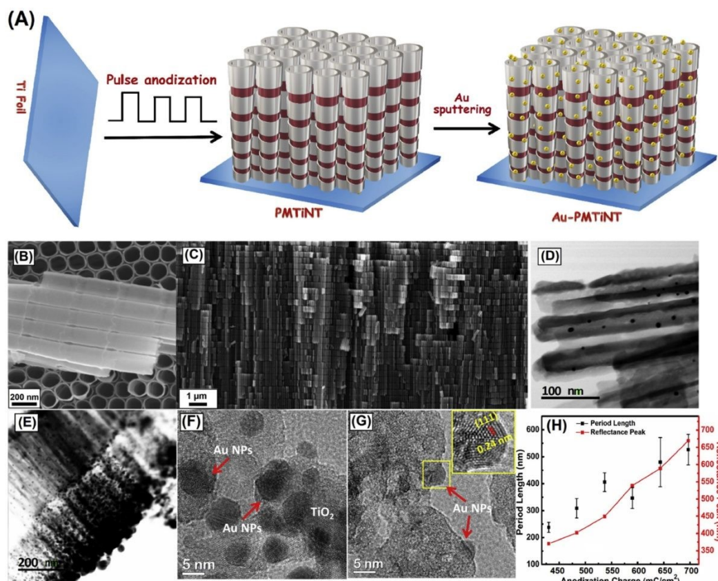
Fig. 7 (A) Schematic illustration of the fabrication process for PMTiNT arrays. (B, C) Top-view and cross-sectional FESEM images of the as-prepared PMTiNT structure, respectively. (D, E) TEM images of Au-loaded PMTiNT, showing the distribution of gold nanoparticles. (F, G) HRTEM images highlighting the gold nanoparticles and their lattice fringes. (H) Dependence of the photonic crystal pitch (defined as the length of the repeating periodic segment) and the corresponding optical reflectance peak on the anodization charge, demonstrating the tunability of photonic bandgaps through charge-controlled anodization. Reproduced with permission from ref. 92. Copyright 2020 Elsevier.
