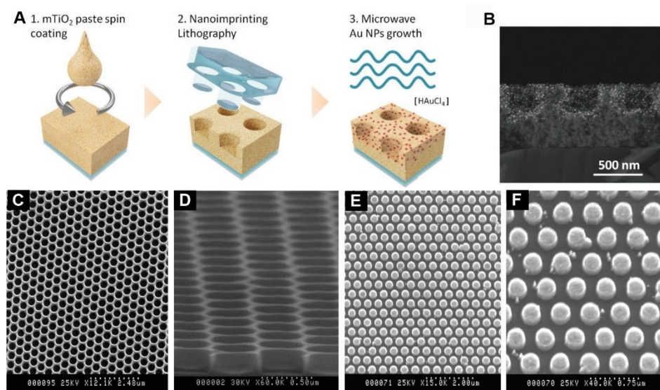
Fig. 6 (A) Fabrication scheme and (B) SEM cross-sectional image of the nanostructured photocatalytic TiO 2 photonic crystal substrates formed by using lithography approach. Reproduced with permission from ref. 50. Copyright 2021 Wiley. SEM images of (C, D) silicon on insulator photonic crystal with 500 nm lattice constant and (E, F) silicon nanoimprint mold fabricated by electron beam lithography. Reproduced with permission from ref. 94. Copyright 2004 Elsevier.
