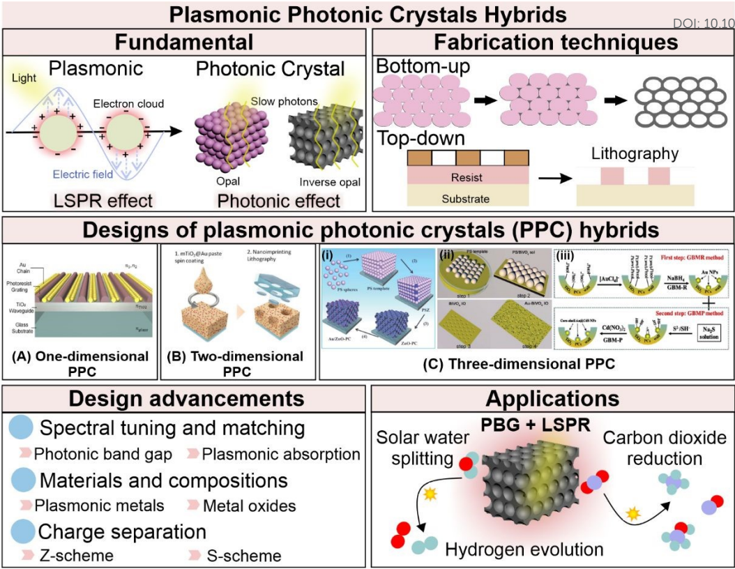
Fig. 1 Overview of plasmonic–photonic crystal (PPC) photocatalysts, from fundamentals to energy applications. (A) Schematic illustration of one-dimensional PPC hybrid, where plasmonic nanoparticle gratings are self-assembled within a photoresist template on a TiO 2 waveguide. Reproduced with permission from ref. 49. Copyright 2019 American Chemical Society. (B) Schematic illustration of two-dimensional PPC hybrid based on a fabrication scheme involving nanostructured photocatalytic substrates integrated with ex situ grown Au nanoparticles. Reproduced with permission from ref. 50. Copyright 2021 Wiley. (C) Schematic illustration of three-dimensional PPC hybrids. (i) Au/ZnO photonic crystal hybrid fabricated via four steps: 1. self-assembly of polystyrene (PS) spheres into a face-centered cubic structure, 2. infiltration with ZnO precursor, 3. drying and calcination, and 4. sputtering of Au nanoparticles onto the ZnO-PC. Reproduced with permission from ref. 51. Copyright 2015 Royal Society of Chemistry. (ii) Au nanocrystal-decorated BiVO 4 inverse opal (IO) fabricated through: 1. monolayer PS sphere self-assembly at the BiVO 4 sol-air interface, 2. transfer onto ITO glass, 3. annealing to form BiVO 4 IO, and 4. thermal evaporation of Au nanocrystals. Reproduced with permission from ref. 52. Copyright 2021 Royal Society of Chemistry. (iii) Au@CdS core-shell nanoparticles supported on an inverse opal TiO 2 scaffold, synthesized via a two-step gas bubbling-assisted membrane reduction-precipitation (GBMR/P) method. Reproduced with permission from ref. 53. Copyright 2015 Elsevier.
