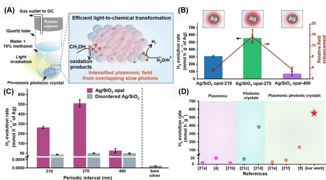
Fig. 11 (A) Schematic illustration of the photoreactor setup using the Ag/SiO 2 opal as plasmonic catalysts for HER. (B) HER and the relative field enhancement observed from various plasmonic PC with different opal diameters. The inset depicts electromagnetic field strength observed for various plasmonic photonic catalysts. (C) H 2 evolution rate from water when in presence of Ag/SiO 2 opals, disordered Ag/SiO 2 platforms, or bare Ag nanoparticles under light irradiation. (D) Comparison of photocatalytic H 2 production rates between the optimized plasmonic-photonic catalytic architecture and other emerging photocatalyst designs
