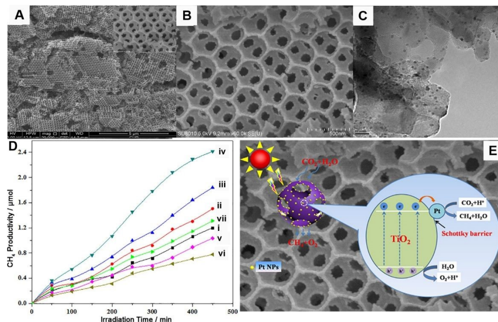
Fig. 9 SEM images of (A) PC-TiO 2 and (B) Pt 4 /PC-TiO 2 . (C) TEM image of Pt 4 /PC-TiO 2 . (D) CH 4 production amounts of P25 and the Pt x /PC-TiO 2 catalysts: i. Pt 0.5 /PC-TiO 2 , ii. Pt 1 /PC-TiO 2 , iii. Pt 2 /PC-TiO 2 , iv. Pt 4 /PC-TiO 2 , v. PC-TiO 2 , vi. P25, and vii. particle-type Pt 4 /TiO 2 . (E) Proposed mechanism of the enhanced photocatalytic activity of Pt x /PC-TiO 2 . Reproduced with permission from ref. 120. Copyright 2017 Wiley.
