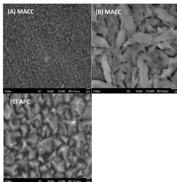
Fig. 3 Displays SEM micrographs of about 5 μm thick Mg resulting from galvanostatic plating of Mg onto a Pt working electrode at 1 mA cm −2 . 0.25 M MACC 2:1 solution in DME is shown at lower and higher magnification in 3A and 3B, respectively. 3C results from 0.25 M APC 2:1 under the same conditions.
