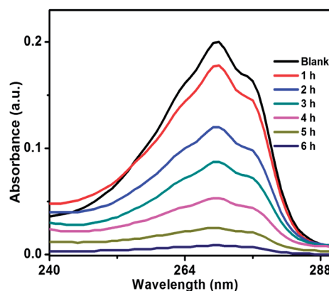
Fig. 11 UV-vis spectrum of decomposition of phenol using ZnO/Au catalyst, under irradiation of visible light. Conditions: [phenol] = 2 \times 10^{-4} \text{ M} and amount of catalyst = 50 mg.
