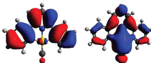
Fig. 2 HOMO (left) and LUMO (right) of [(C N^N^C )Au(CO)] + as simulated by DFT.
