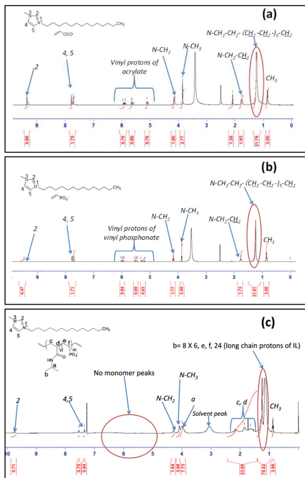
Fig. 2 ^1\text{H} -NMR spectra of ionic liquids and random copolymers (a) 1-tetradecyl-3-methylimidazolium acrylate (TDMIAC), (b) 1-tetradecyl-3-methylimidazolium vinylphosphonate (TDMIACVP) and (c) PNIPAM-co-PTDMIACVP (5 mol% AIBN).
