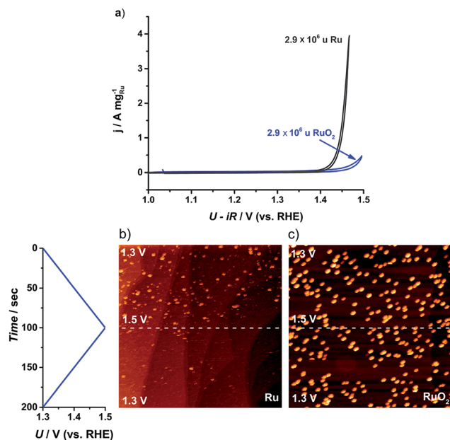
Fig. 5 (a) Cyclic voltammogram (CV) for the first cycle of the as-deposited Ru and thermally oxidized RuO 2 2.9 \times 10^6 u nanoparticles on GC. CV recorded in N 2 saturated 0.05 M H 2 SO 4 between 1.0 and 1.5 V (vs. RHE) at 20 mV s -1 and 1600 rpm. (b) and (c) Potentiodynamic STM images of Ru dissolution in Ar-saturated 0.05 M H 2 SO 4 solution. The potential was scanned between 1.3 and 1.5 V (vs. RHE) at 2 mV s -1 : (b) 0.001 monolayer of as-deposited 0.1 \times 10^6 u Ru nanoparticles, (520 nm) 2 U_B = -299 mV, I_T = 1 nA; (c) 0.001 monolayer of thermally treated 0.1 \times 10^6 u RuO 2 nanoparticles, (516 nm) 2 U_B = -245 mV, I_T = 1 nA.
