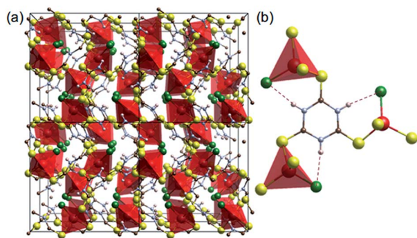
Fig. 1 Crystal structure of [\text{CuCl}(\text{ttcH}_3)] . 13 (a) 2 \times 2 \times 2 cells. (b) Connectivity of \text{CuCl}_3 tetrahedral with the thioketone form of tri-thiocyanuric acid molecules (red: Cu, green: Cl, yellow: S, blue: N, brown: C, and white: H). Dotted lines show hydrogen bonding.
