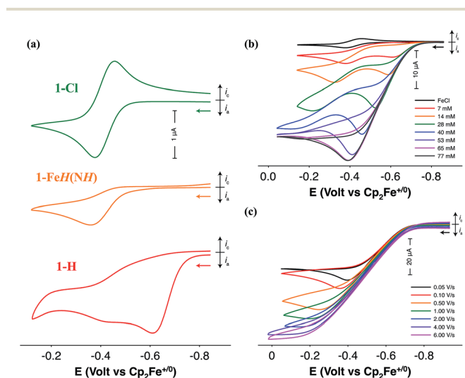
Fig. 2 (a) CVs of 1-Cl (green), 1-FeH(NH) (orange), and 1-H (red) in fluorobenzene solution at 50 mV s -1 . (b) CVs of a fluorobenzene solution of 1-FeH(NH) upon addition of DABCO under 1 atm H 2 at 50 mV s -1 . The initial CV (black) corresponds to 1-Cl prior to activation with NaBAR 4 F . (c) CVs of a fluorobenzene solution of 1-H in the presence of 77 mM DABCO under 1 atm H 2 as a function of scan rate. Conditions for all experiments: 1 mM [Fe], 0.1 M [ᵀBu 4 N][B(C 6 F 5 ) 4 ], 22 °C.
