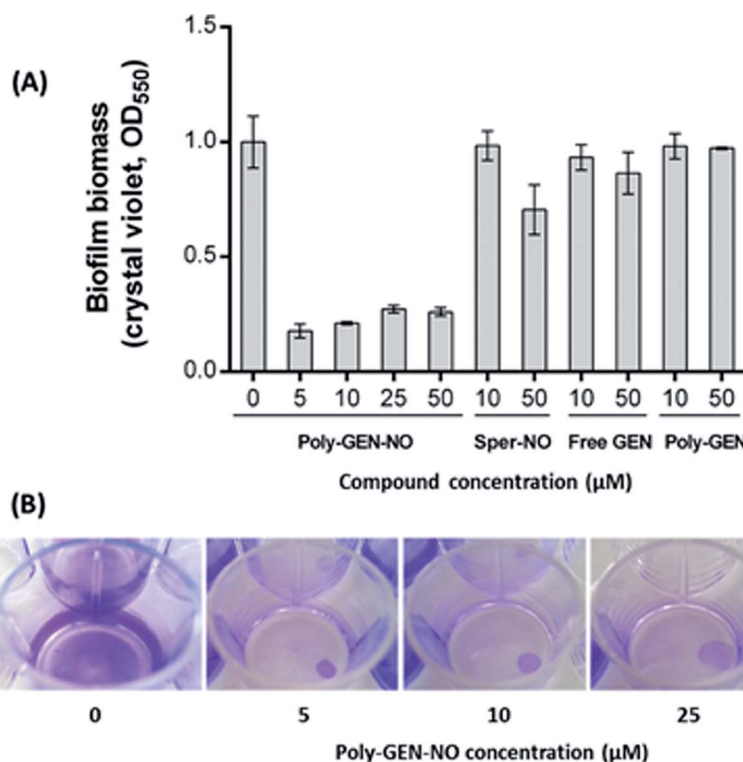
Fig. 5 GEN-NO nanoparticles induced dispersal in P. aeruginosa biofilms. (A) Bacterial biofilms were grown in multi-well plates for 6 h in the absence of any treatment before being treated for a further 1 h with various concentrations (μM) of NO donor spermine NONOate (Sper-NO), free gentamicin or gentamicin-conjugated polymers (Poly-GEN) and GEN-NO nanoparticles (Poly-GEN-NO). Biofilm biomass was analyzed by crystal violet staining. Error bars represent standard error ( n = 2 ). (B) Stained biofilms treated with the indicated concentrations of GEN-NO nanoparticles. Note: concentration based on GEN, one mole of GEN-NO nanoparticles is equivalent to one mole of Sper-NO and gentamicin.
