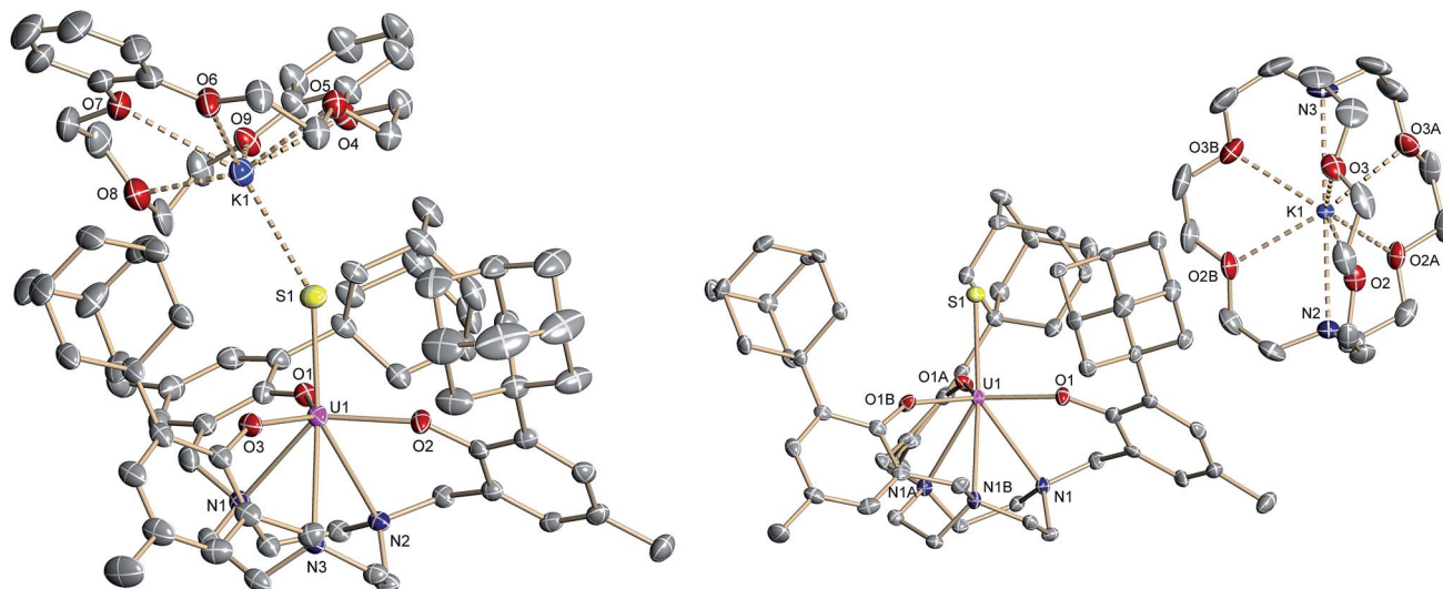
Fig. 2 Molecular structure of the uranium(IV) sulfido complex [(\text{Ad}^{\text{Me}}\text{ArO})_3\text{tacn}]\text{U}\equiv\text{S}\cdots\text{K}(\text{db-18-c-6}) ( 3 ) (left), and [\text{K}(\text{2.2.2-crypt})][(\text{Ad}^{\text{Me}}\text{ArO})_3\text{tacn}]\text{U}\equiv\text{S} ( 4 ) (right). All hydrogen atoms and the solvent molecules are omitted for clarity (50% probability ellipsoids).
