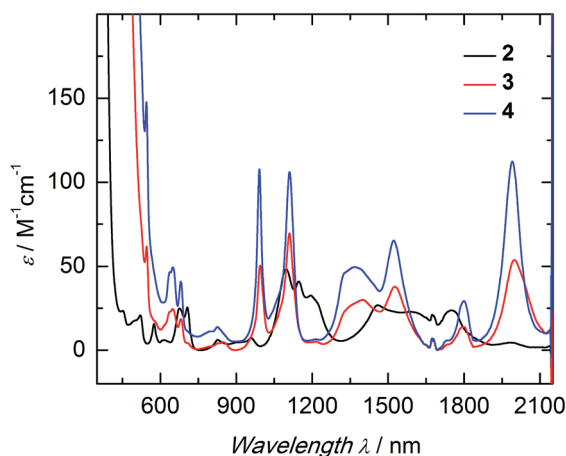
Fig. 3 Electronic absorption spectra of the uranium hydrosulfido complex [(^{\text{Ad,Me}}\text{ArO})_3\text{tacn}]\text{U}-\text{SH} (2, black) and terminal sulfido complexes [(^{\text{Ad,Me}}\text{ArO})_3\text{tacn}]\text{U}\equiv\text{S}\cdots\text{K}(\text{db-18-c-6}) (3, red) and [\text{K}(2.2.2\text{-crypt})][(^{\text{Ad,Me}}\text{ArO})_3\text{tacn}]\text{U}\equiv\text{S} (4, blue); all complexes 5 mM in pyridine, measured at RT.
