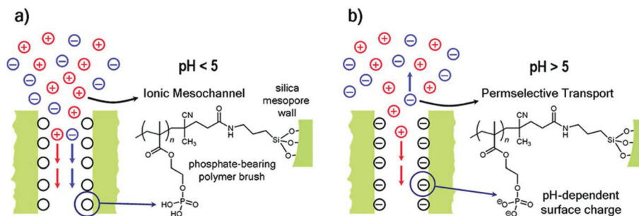
Fig. 22 Schematic depiction of the ionic transport processes taking place in the hybrid polymer–inorganic interfacial assembly at different pH values: (a) \text{pH} < 5 , ionic mesochannel (no exclusion of ionic species) and (b) \text{pH} > 5 , permselective transport of cations (Copyright 2012, The American Chemical Society, reprinted from ref. 247).
