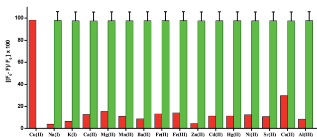
Fig. 4 Fluorescence Quenching Efficiency (FQE) of H 5 dpm ( 5 \times 10^{-6} M) in Tris buffer solution (25 mM, pH = 7.4) in the presence of 100 μM of different types of metal ions except Cu 2+ (50 μM) as a bar graph [the red bar portion]. Fluorescence Quenching Efficiency (FQE) of a mixture of H 5 dpm ( 5 \times 10^{-6} M) solution with other metal ions (100 μM) followed by addition of 50 μM Cu 2+ to the solution [the green bar portion] ( \lambda_{\text{ex}} = 434 nm, \lambda_{\text{em}} = 510 nm, slit: 5 nm/5 nm).
