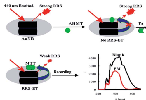
Fig. 25 Schematic of RRS-ET method for detection of FA (this figure has been adapted from ref. 75 with permission from Springer).
