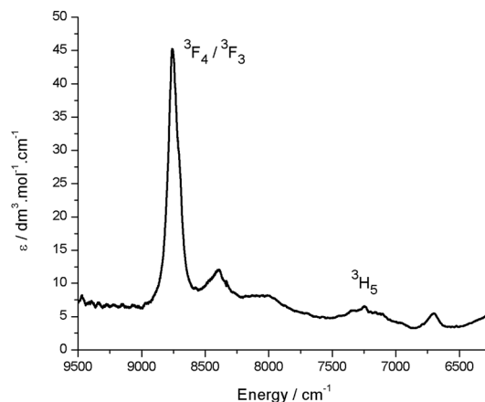
Fig. 5 Room temperature NIR absorption spectrum for 3 (toluene solution). Assignments are based on comparison with \text{U(IV)} pentahalide anions, which display near-identical NIR spectra. 45
