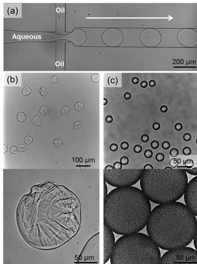
Fig. 6 Transmission optical micrographs. (a) An example flow-focussing junction resulting in monodisperse microdroplets, typically with flow rates of 150 and 100 \mu L h^{-1} for the oil and water flows respectively; (b) top panel shows aqueous microdroplets containing A_2-B_3-CB[8] and continuous FC-40 oil containing 2 wt% XL171 and 1 wt% K^+ , and bottom panel is at higher magnification; (c) top panel shows aqueous microdroplets containing A_2-B_3-CB[8] and continuous FC-40 oil containing 2 wt% XL171 and 1 wt% K^+ , and bottom panel is at higher magnification.
