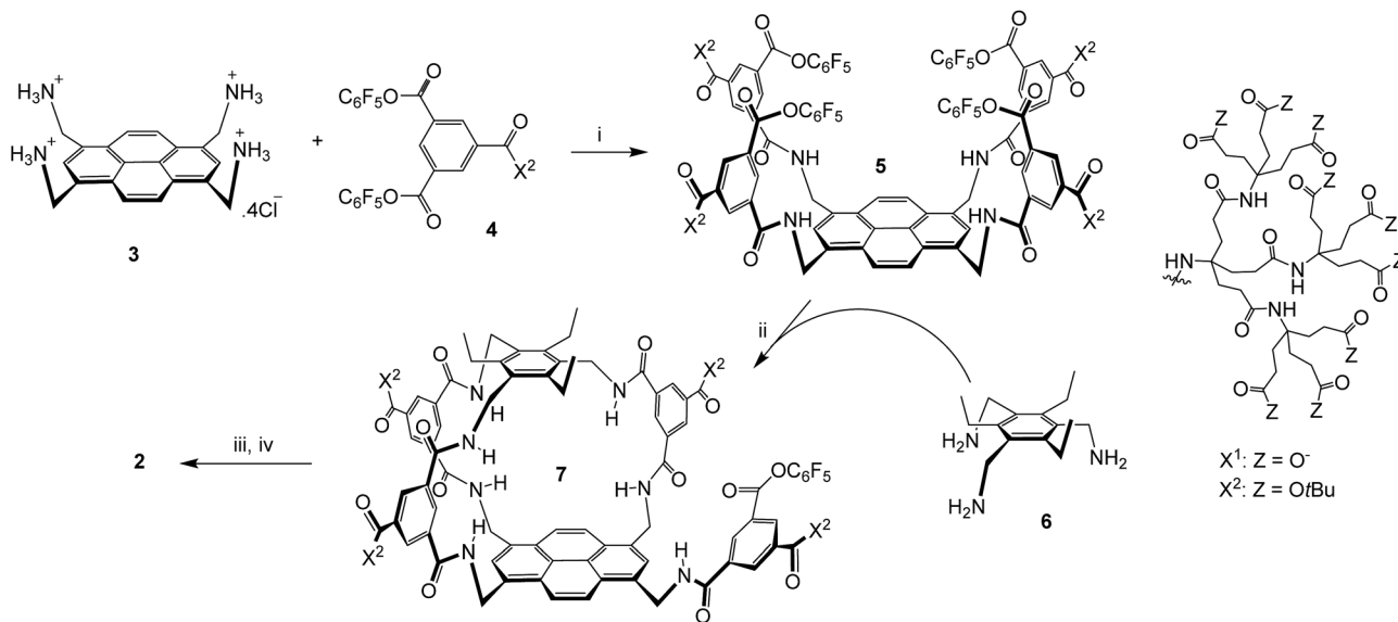
Scheme 1 Synthesis of (±)-2. (i) THF/water, 4 (8 equivalents), \text{EtN}(\text{iPr})_2 , 47%; see ref. 14a. (ii) THF, \text{EtN}(\text{iPr})_2 , [5] and [6] \leq 0.11 mM, 51%. (iii) TFA, DCM. (iv) NaOH, \text{H}_2\text{O} , then Amberlyst 15 hydrogen form, then NaOH (to pH = 7).
