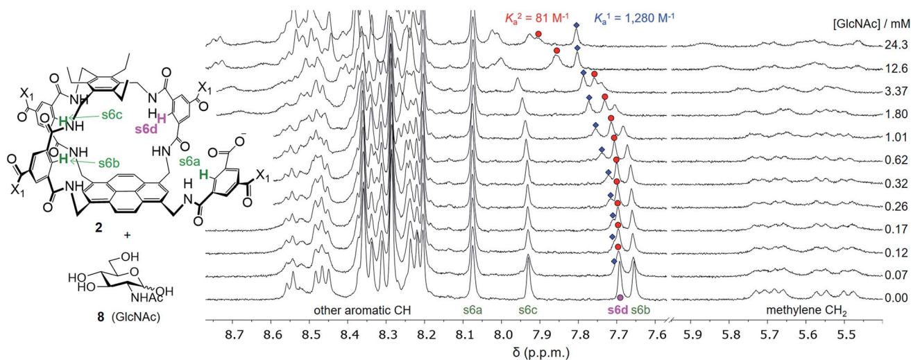
Fig. 3 Selected partial spectra for a ^1\text{H} NMR binding study of receptors (±)- 2 (0.15 mM each) with D-GlcNAc 8 in \text{D}_2\text{O} . The labelling system used for 2 and a full NMR assignment are detailed in the ESI.† Signals due to protons s6a–d appear in the region 7.6–8.1 ppm and are readily observed during the titration. In particular, the signal due to s6d splits into two peaks which can be followed throughout.
