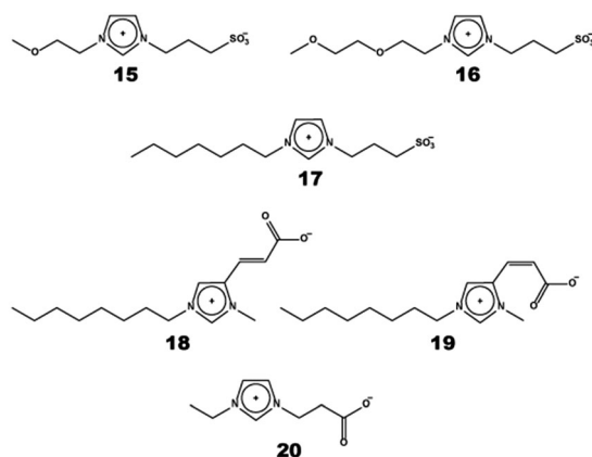
Fig. 6 Chemical structure of ZIs.
