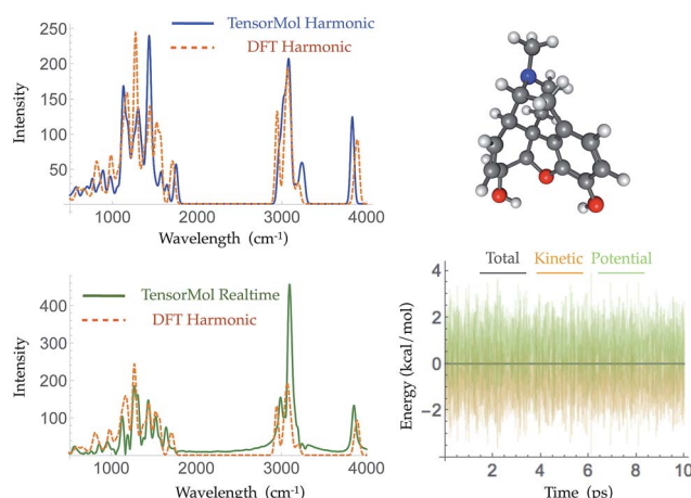
Fig. 7 The geometry of morphine as optimized by TensorMol-0.1 (upper right panel) and its harmonic IR spectra simulated using \omega\text{B97X-D/6-311G}^{**} (dashed orange line) and the TensorMol force field (solid blue line) (upper left panel). The lower panels show the real-time IR spectra obtained using TensorMol (solid green line), and the DFT results (dashed orange line) (left), and the conservation of energy maintained by the smoothness of the energy (right).
