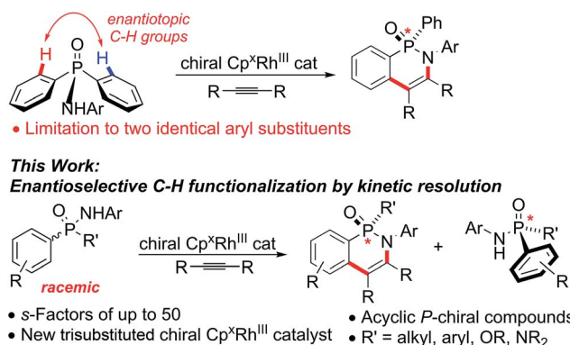
Scheme 1 \text{Rh}^{\text{III}} -catalyzed desymmetrization and kinetic resolution approaches for the synthesis of P-chiral compounds.
