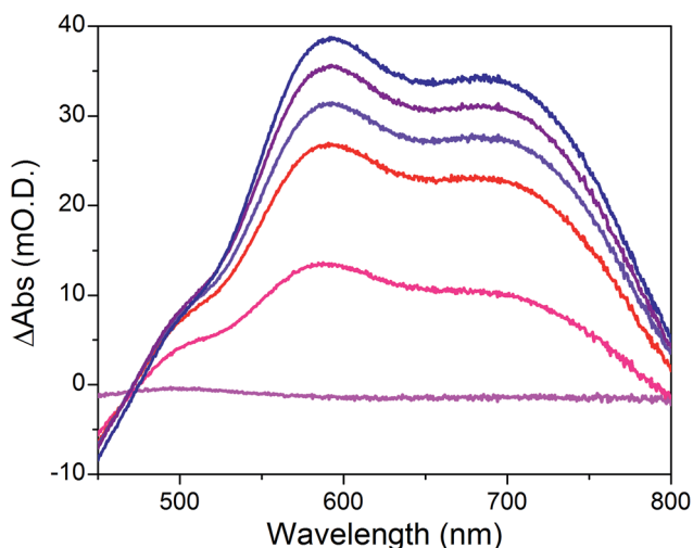
Fig. 9 Differential UV-visible spectra of a \text{NiO|Co}_{\text{C11P}} electrode poised in a NaCl 0.1 M aqueous electrolyte at -0.44 (magenta line), -0.54 (pink line), -0.64 (red line), -0.74 (violet line), -0.84 (purple line) and -0.94 (navy blue line) V vs. NHE, with subtraction of the spectrum of the same electrode poised at -0.34 V vs. NHE under identical conditions.
