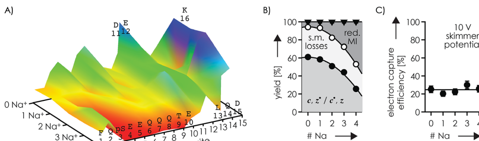
Fig. 3 (A) Site-specific fragmentation efficiency ( c , z' and c' , z fragments) from ECD of phosphopeptide ions with a net charge of 3+ and 0-4 \text{Na}^+ ions attached, with the color scale ranging from red (zero fragmentation) to yellow to green to blue (maximum fragmentation; detailed fragmentation efficiency values can be found in Fig. S7A and B†); (B) percentage stacked area plots illustrating the yield of c , z' and c' , z fragments, products from loss of small molecules (s.m.) from reduced molecular ions, and reduced molecular ions (including loss of \text{H}^+ ; loss of \text{Na}^+ was not observed) from ECD of phosphopeptide ions with a net charge of 3+ at 10 V skimmer potential, and (C) corresponding electron capture efficiency versus the number of \text{Na}^+ ions attached; solid lines in (B) are quadratic polynomial functions used for error analysis and that in (C) is meant to guide the eye.
