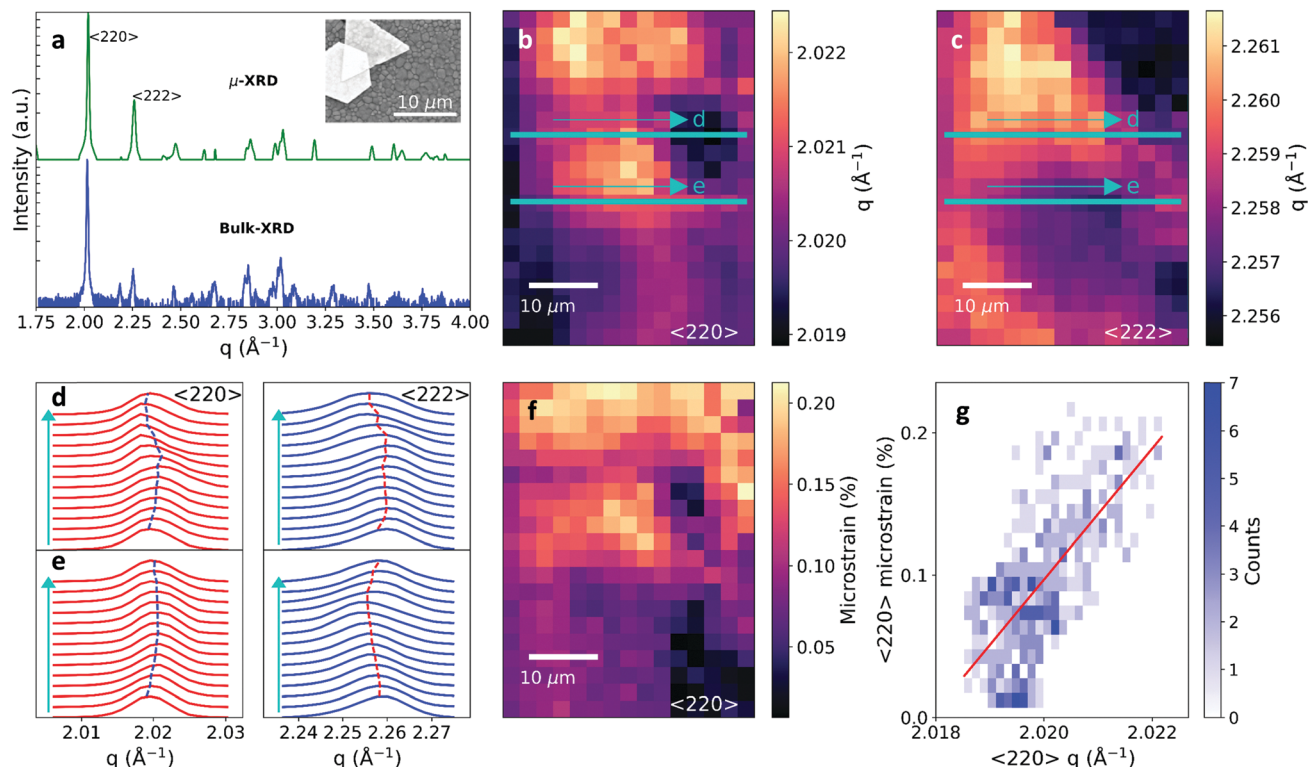
Fig. 1 Characterising structural heterogeneity in MAPbI 3 films on glass cover slips by μXRD. (a) Comparison of the macroscopic bulk XRD pattern with the μXRD pattern (both collected at 240 K) summed over a 70 × 70 μm 2 spatial region, with the key reflections labelled. Inset: SEM image of the perovskite grains along with ~ten-micrometer-sized Au fiducial marker particles. (b) Local <220> and (c) <222> diffraction peak q maps revealing substantial structural heterogeneity. (d and e) Selected slices of the <220> (red) and <222> (blue) through the maps in (b and c) illustrating the complex strain patterns present within the film. Vertical lines indicate peak position as determined through peak profile fitting and are a guide to the eye. (f) Microstrain map for the <220> diffraction peak. (g) Histogram of the calculated microstrain and corresponding scattering vector q for the <220> diffraction peak. The solid line is a linear regression fit to a scatter plot of the data, revealing a statistically-significant correlation (negligible p -value; see Methods).
