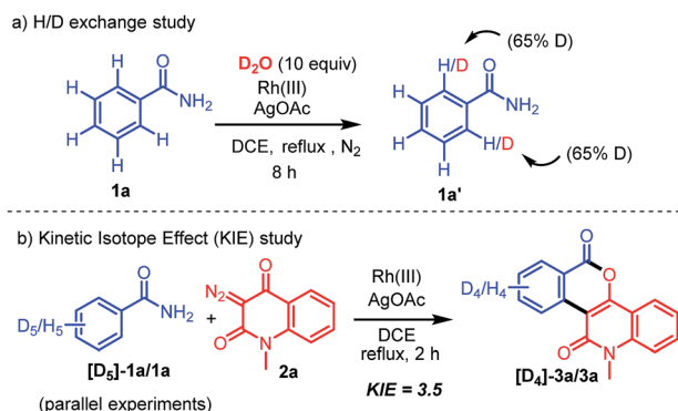
Scheme 5 Deuterium labelling experiments.
