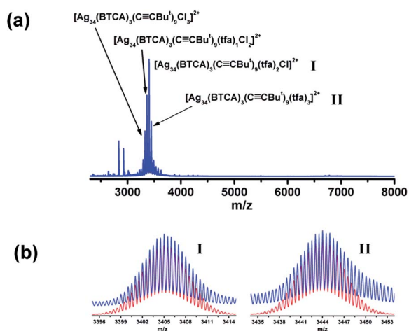
Fig. 2 (a) Mass spectrum of cluster 1. (b) The measured (blue trace) and simulated (red trace) isotopic patterns of [\text{Ag}_{34}(\text{BTCA})_3(\text{C}\equiv\text{CBu}^t)_9(\text{tfa})_2\text{Cl}]^{2+} (I) and [\text{Ag}_{34}(\text{BTCA})_3(\text{C}\equiv\text{CBu}^t)_9(\text{tfa})_3]^{2+} (II).
