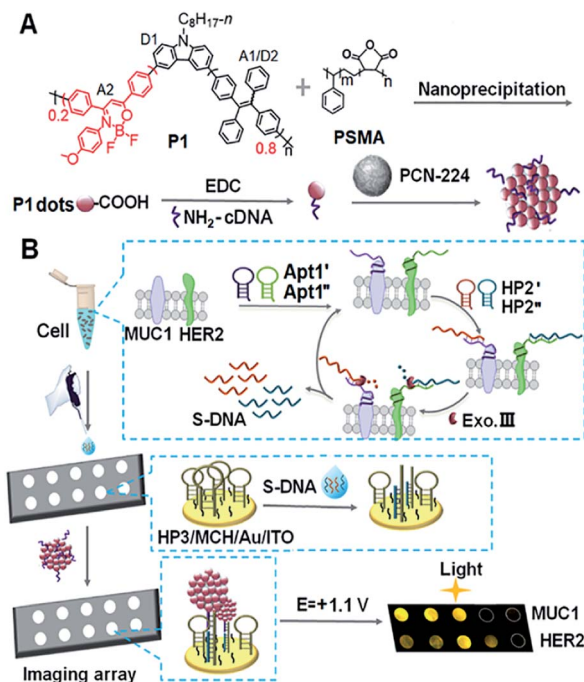
Scheme 1 Schematic diagram of (A) preparation of Pdets@PCN-224 as an ECL probe and (B) ECL imaging array for the analysis of two kinds of membrane proteins with target-mediated cyclic amplification.
