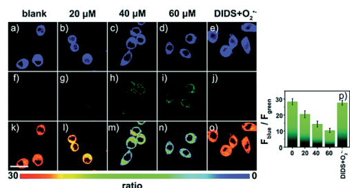
Fig. 11 Confocal fluorescence images of RAW264.7 cells stained with 5 \mu M 17 under different treatments: (a, f and k) control; (b, g and l) 20 \mu M O_2^{\bullet-} ; (c, h and m) 40 \mu M O_2^{\bullet-} ; (d, i and n) 60 \mu M O_2^{\bullet-} ; (e, j and o) 100 \mu M DIDS + 60 \mu M O_2^{\bullet-} . (p) The corresponding F_{blue}/F_{green} . Adapted with permission from ref. 43b. Copyright 2018 Royal Society of Chemistry.
