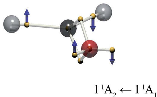
Fig. 4 The electron positions for the mid-point of the vibration, \bar{x} = (\bar{x}_i + \bar{x}_f)/2 , and the displacement vector \mathbf{x}_{fi} for the wavefunction mixed between the 1^1A_1 (ground), and 1^1A_2 , 2^1A_1 and 1^1B_1 excited states of formaldehyde. The vector length is doubled for clarity.
