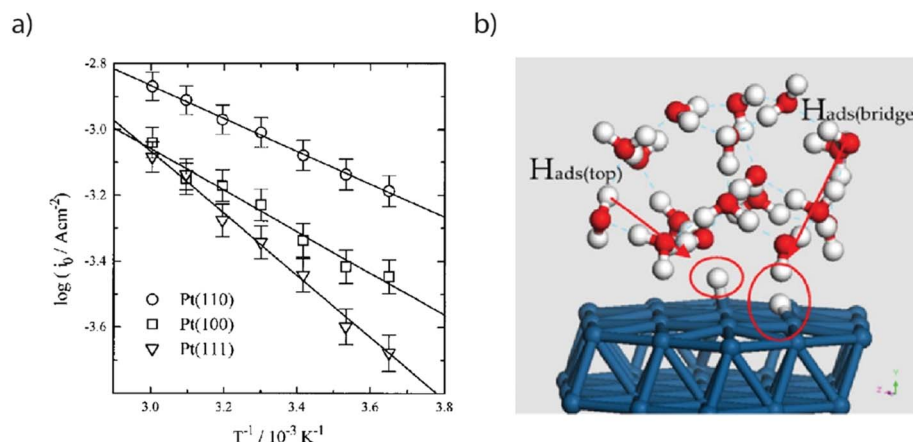
Fig. 2 (a) Arrhenius plot of exchange current densities for Pt(110) (circle), Pt(100) (square) and Pt(111) obtained by cyclic voltammetry in a 50 mM H 2 SO 4 solution (reproduced from ref. 21 with permission from the American Chemical Society, Copyright (1997)). (b) Snapshot of a MD-DFT simulation showing the presence of two types of adsorbed hydrogen on a Pt(111) electrode. Reproduced from ref. 23 with permission from Elsevier, Copyright (2007).
