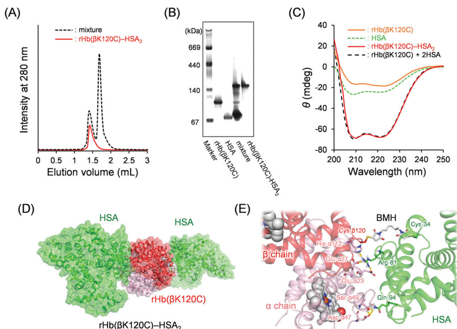
Fig. 3 (A) SEC profiles of the resultant reaction mixture [rHb(βK120C) + MA-HSA] and the purified rHb(βK120C)–HSA 2 trimer. (B) Native PAGE patterns of rHb(βK120C), HSA, the reaction mixture, and the purified rHb(βK120C)–HSA 2 trimer. (C) CD spectra of rHb(βK120C), HSA, rHb(βK120C), and rHb(βK120C)–HSA in PBS at 25 °C ([protein] = 0.2 μM). (D and E) The energy-minimized structure of the rHb(βK120C)–HSA 2 trimer obtained by a molecular dynamics (MD) calculation using the Desmond software.
