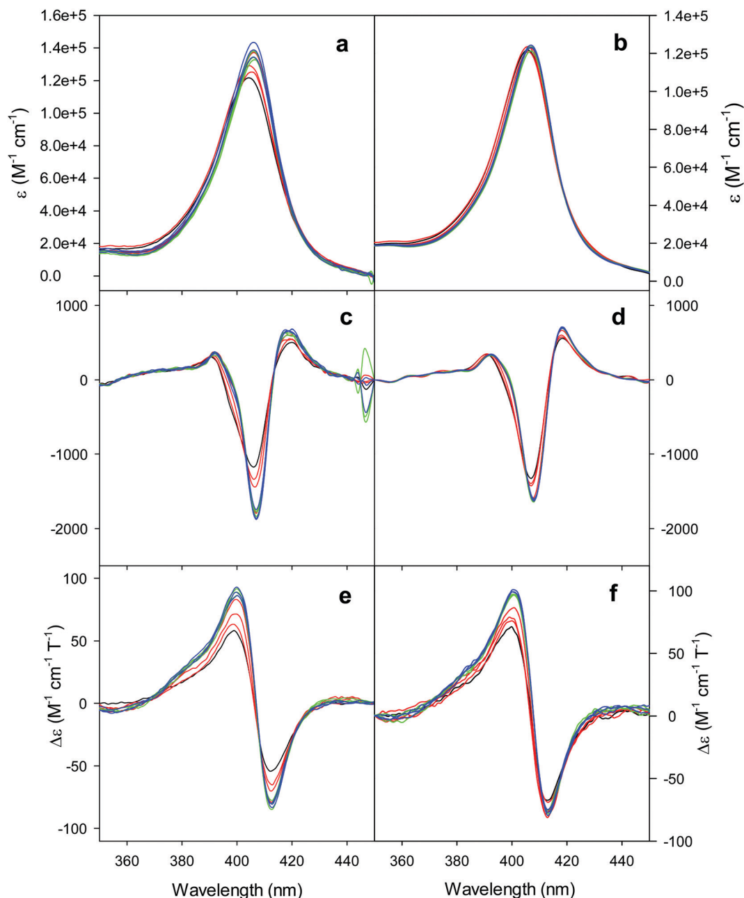
Fig. 2 Electronic absorption, 2nd derivative electronic absorption and MCD spectra in the Soret region for the oxidized M80A (a, c and e) and M80AY67A (b, d and f) variants of S. cerevisiae iso-1 cytochrome c in 5 mM phosphate buffer at pH 7 in the presence of increasing urea concentration: 0 M (black); 1, 2, and 3 M (red); 4, 5, and 6 M (green); and 7, 8, and 9 M (blue).
