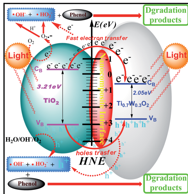
Scheme 1 Proposed phenol photocatalytic degradation mechanism at the \text{Ti}_{0.7}\text{W}_{0.3}\text{O}_2/\text{TiO}_2 NCI.
