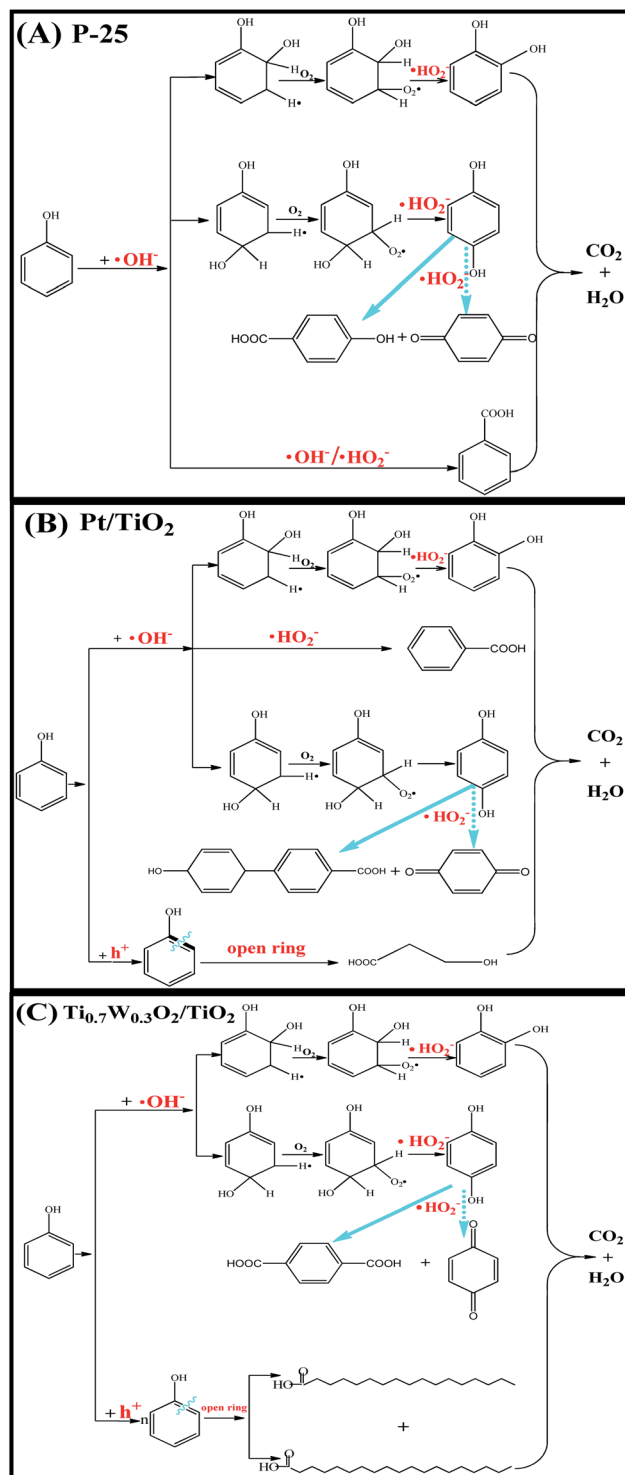
Fig. 9 Proposed photocatalytic degradation process of phenol over: (A) P-25, (B) Pt/TiO 2 and (C) Ti 0.7 W 0.3 O 2 /TiO 2 NCl.
