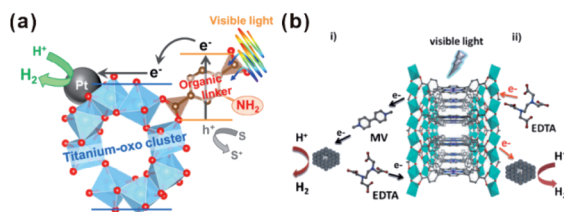
Fig. 22 Scheme illustrating the photocatalytic \text{H}_2 production reaction over (a) Pt/Ti-MOF- \text{NH}_2 and (b) Al-PMOF based on LCCT or LCMT mechanisms. Reproduced with permission. 203 Copyright©2012, 2015 American Chemistry Society. Reproduced with permission. 204 Copyright©2012 WILEY-VCH Verlag GmbH & Co. KGaA.
