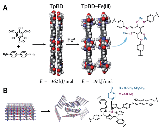
Fig. 20 Coordination-induced chemical exfoliation of COFs. (A) Fe 3+ -assisted aqueous-phase chemical exfoliation to prepare TpBD COF nanosheets. Adapted under a Creative Commons Attribution 4.0 International License. Copyright 2018, The Author(s). 175 Published by Springer Nature Limited. (B) Porphyrin-based nanodisks synthesized via the simultaneous axial coordination of pyridines and metal ions. Adapted under a Creative Commons Attribution 4.0 International License. Copyright 2019, The Author(s). 176 Published by Springer Nature Limited.
