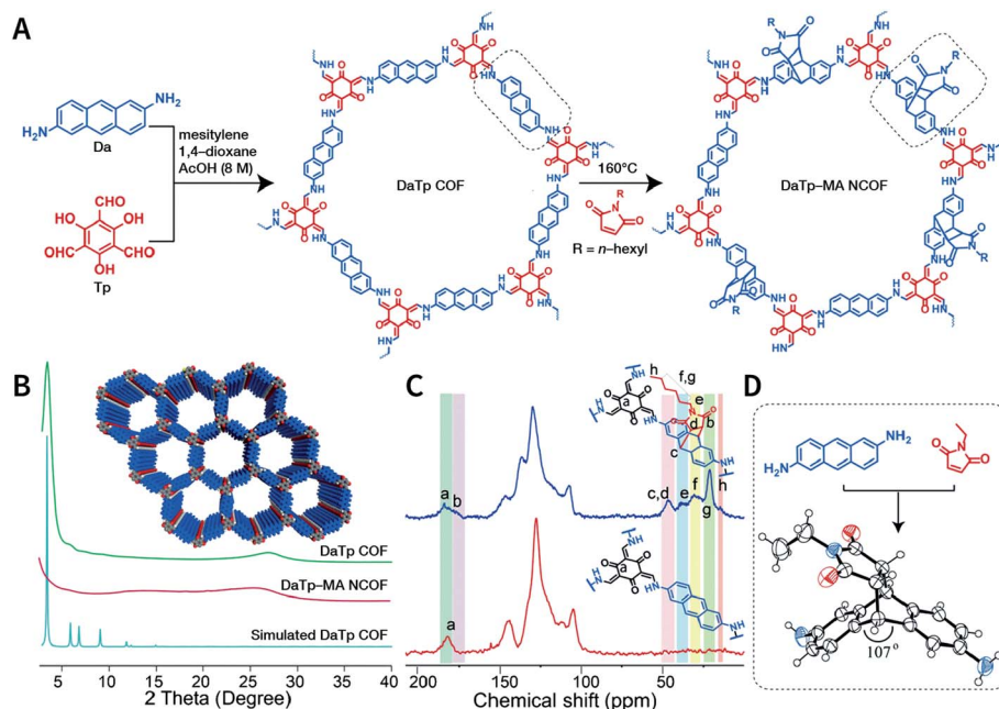
Fig. 19 Synthesis of DaTp-MA NCOF sheets through the Diels–Alder cycloaddition-induced chemical exfoliation. (A) Reaction formula of COF preparation and chemical exfoliation. (B) PXRD patterns. (C) 13 C solid-state NMR spectra of DaTp COF (red) and DaTp-MA NCOF (blue). (D) Model compound synthesized from 2,6-diaminoanthracene and N -ethylmaleimide. Adapted with permission. 173 Copyright 2016, Wiley-VCH Verlag GmbH & Co. KGaA, Weinheim.
