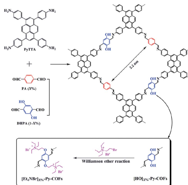
Fig. 46 Williamson ether synthesis of IL-functionalized [\text{Et}_4\text{NBr}]_{\text{X}\%}\text{-Py-COFs} for catalyzing the formylation reaction. Adapted with permission. 305 Copyright 2016, The Royal Society of Chemistry.
