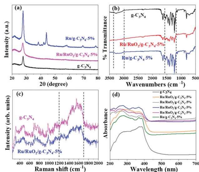
Fig. 1 XRD patterns (a), FTIR spectra (b), Raman spectra (c), and UV-Vis spectra (d) of g\text{-C}_3\text{N}_4 , Ru/RuO 2 / g\text{-C}_3\text{N}_4 -5% and Ru/ g\text{-C}_3\text{N}_4 -5%.
