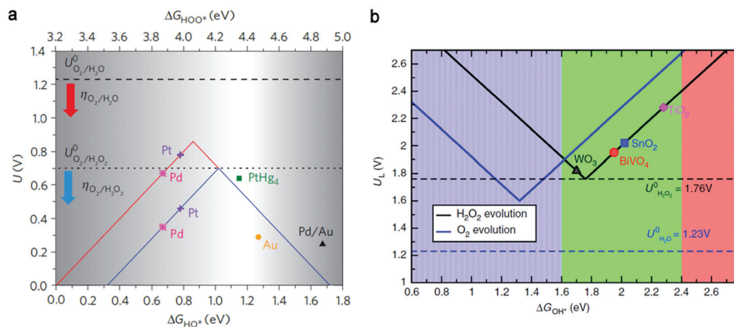
Fig. 3 (a) Calculated oxygen reduction volcano plot for the two-electron (blue) and four-electron (red) reduction of \text{O}_2 , with the limiting potential plotted as a function of \Delta G_{\text{HO}^*} (lower horizontal axis) and \Delta G_{\text{HOO}^*} (upper horizontal axis). The equilibrium potentials for the two-electron and four-electron pathway are shown as the dotted line and dashed line, respectively. The range of interesting \text{OH}^* free energy for high selectivity and activity is highlighted with the greyscale gradient at its edges, recognizing limitations to the accuracy of DFT. Reproduced with permission. 33 Copyright 2013 Springer Nature. (b) Activity volcano plots based on calculated limiting potentials as a function of calculated \Delta G_{\text{OH}^*} for the two-electron oxidation of \text{H}_2\text{O} to \text{H}_2\text{O}_2 (black) and the four-electron oxidation to \text{O}_2 (blue). The corresponding equilibrium potentials for each reaction are shown in dashed lines. Reproduced with permission. 41 Copyright 2017 Springer Nature.
