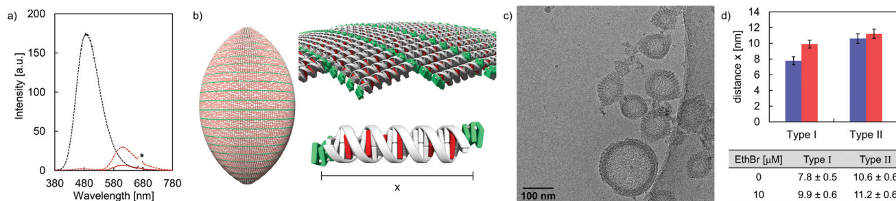
Fig. 6 (a) Fluorescence emission spectra of vesicles assembled from duplex A-B in aqueous medium at 20 °C in the absence (black) and presence of 10 μM EthBr (red). Conditions: 1 μM A-B, 10 mM sodium phosphate buffer pH 7.2, 0.1 mM spermine-4 HCl, 20 vol% ethanol, solid line: \lambda_{\text{ex}} : 520 nm, dotted line: \lambda_{\text{ex}} : 335 nm. (b) Illustration of EthBr (red) intercalation. (c) Cryo-EM image in the presence of 10 μM EthBr. (d) EthBr intercalation leads to a statistically significant widening of the bands in type I vesicles.
