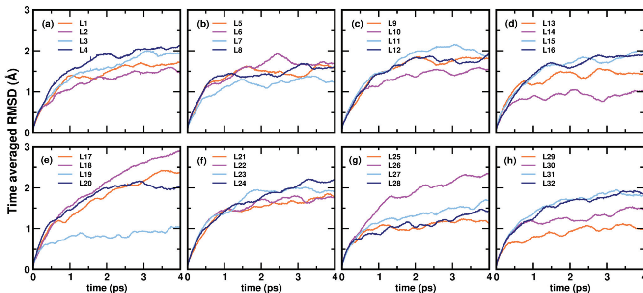
Fig. 3 (a)–(h) Show the time-averaged root-mean-square deviation (RMSD) of every individual ligand in the Au 68 (m-MBA) 32 cluster, after temperature equilibration, as a function of simulation time evaluated at 300 K.
