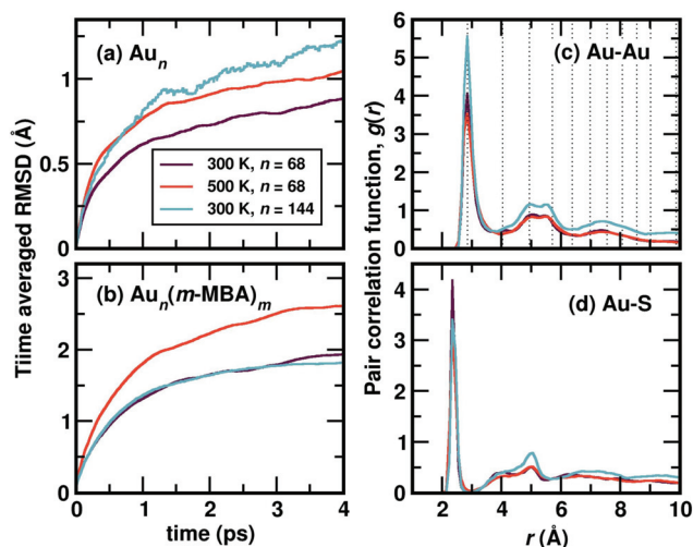
Fig. 2 Time-averaged root-mean-square deviation (RMSD) of Au 68 (m-MBA) 32 and Au 144 (m-MBA) 40 clusters as a function of simulation time after temperature equilibration, evaluated for (a) the gold core and (b) all atoms of the cluster. The pair-correlation function, g(r) , of (c) Au–Au and (d) Au–S pairs, in the two clusters, the 68-atom cluster at 300 K and 500 K and 144-atom cluster at 300 K.
