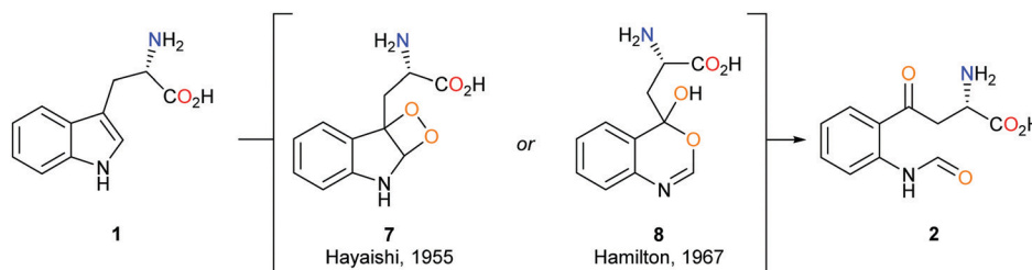
Scheme 2 Hayashi's 7 and Hamilton's 8 proposed metabolic intermediates.
