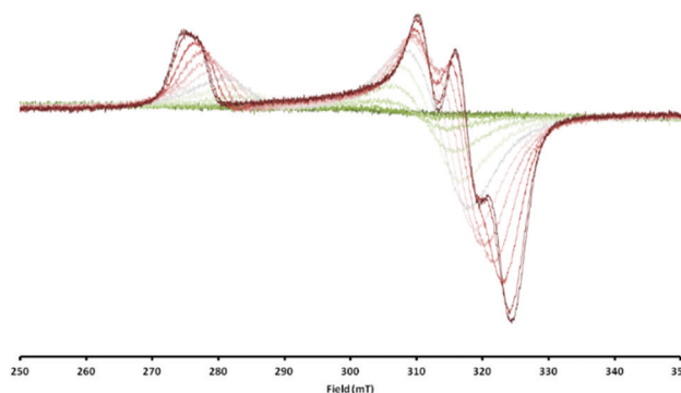
Fig. 3 Overlaid EPR spectra of [L^{tBu}NiBr][Cp_2Co] in toluene measured between 20 °C (dark green, silent) and -95^\circ\text{C} (dark red, up to ~60%).
