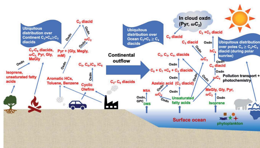
Fig. 4 Schematic representation of atmospheric reaction pathways of dicarboxylic acids and other related water-soluble organic compounds (Ox = photochemical oxidation). Adapted from ref. 162 with permission from Elsevier, © 2016.
