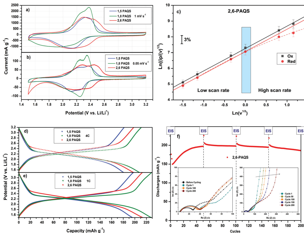
Fig. 4 (a) and (b) Cyclic voltammetry of PAQS isomers with 1 M LiTFSI in DOL/DME at 1.00 and 0.05 mV s⁻¹. (c) Evolution of normalized current ( ip ) as a function of the square root of the scan rate v . (d) and (e) Galvanostatic profiles of each PAQS isomer at 4C and 1C. (f) 2,6-PAQS impedance evolution during galvanostatic cycling at 4C.
