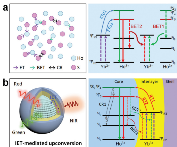
Fig. 1 (a) Left: Schematic of the deleterious quenching interactions between \text{Ho}^{3+} and the sensitizer \text{S} (e.g., \text{Yb}^{3+} ) in a codoping system, in particular at high dopant concentrations. Right: Two typical back energy transfer processes (BET1 and BET2) that may quench the red and green emitting energy levels of \text{Ho}^{3+} for a \text{Ho}^{3+}/\text{Yb}^{3+} codoped system. (b) Proposed mechanistic model (left) and possible ionic interactions (right) when using interfacial energy transfer to activate the holmium sublattice toward the upconversion in a core-shell-shell nanostructure in which the activator and sensitizer are spatially separated into different layers. ETU, BET, IET, and CR stand for energy transfer upconversion, back energy transfer, interfacial energy transfer, and cross-relaxation, respectively.
