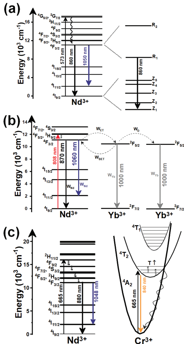
Fig. 21 Mechanisms of generation of the emission lines of: (a) single-doped \text{Nd}^{3+} luminescent thermometers excited at 573 nm, (b) dual emitting center \text{Nd}^{3+}/\text{Yb}^{3+} luminescent thermometers excited at 808 nm, and (c) dual emitting center \text{Nd}^{3+}/\text{Cr}^{3+} luminescent thermometers excited at 665 nm, operating simultaneously in the I- and II-BWs.
