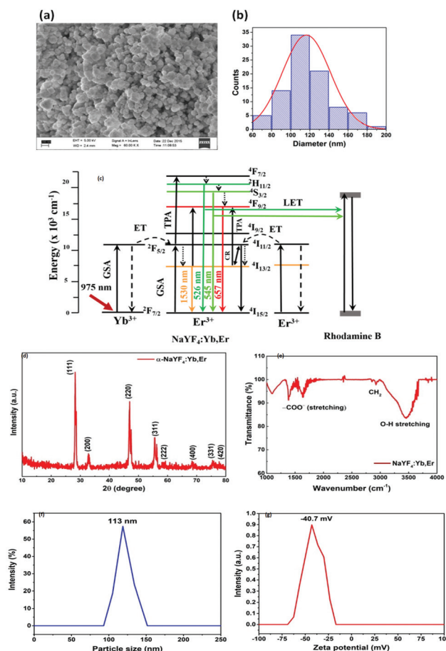
Fig. 4 This figure shows the (a) SEM information for a particle with an average size of 120 nm, (b) the corresponding size distribution and (c) the energy level diagram of the UCNPs. (d) Powder X-ray diffraction patterns for the UCNPs (e) Fourier Transform Infra Red spectra for the UCNPs. These indicate that the UCNPs sample is very pure and homogeneous. (f) The dynamic light scattering data for UCNPs (g) the zeta-potential for the colloidal solution of UCNPs.
